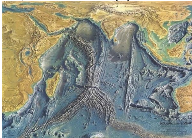
Fig. 1: Sub ocean map of the earth
